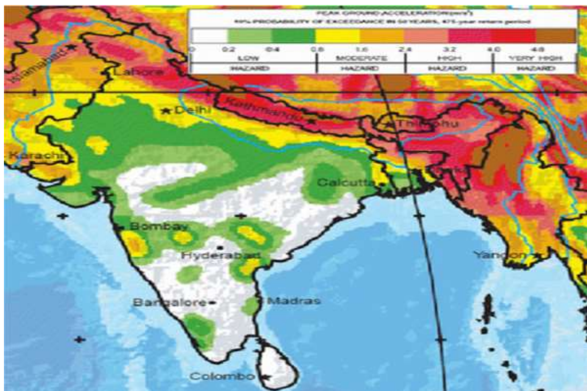
Fig: Seismic Hazard Map of India, the Himalaya and Bangladesh
