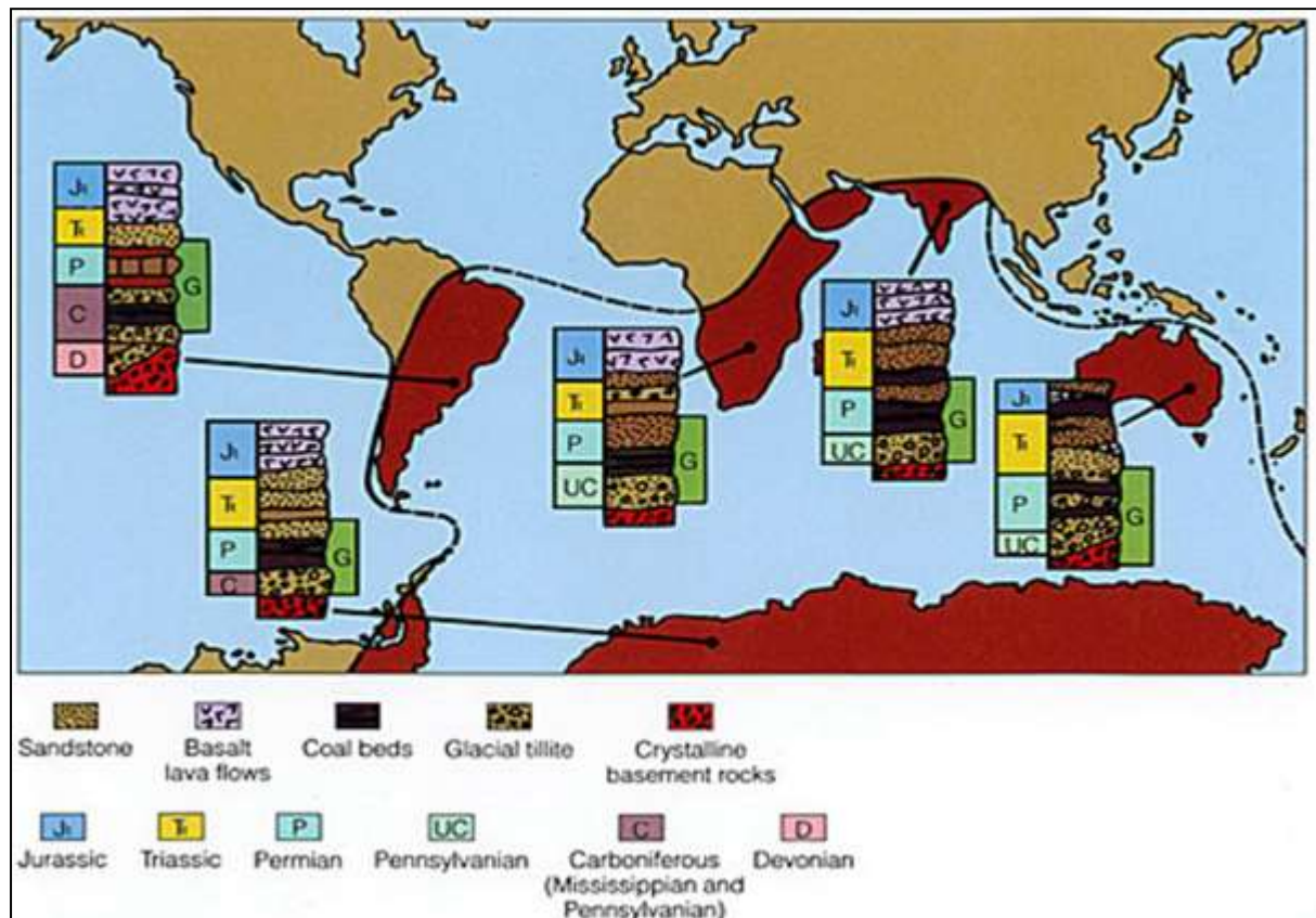
■ Matching glacier deposits - Matching glacier deposits 300 million years ago
