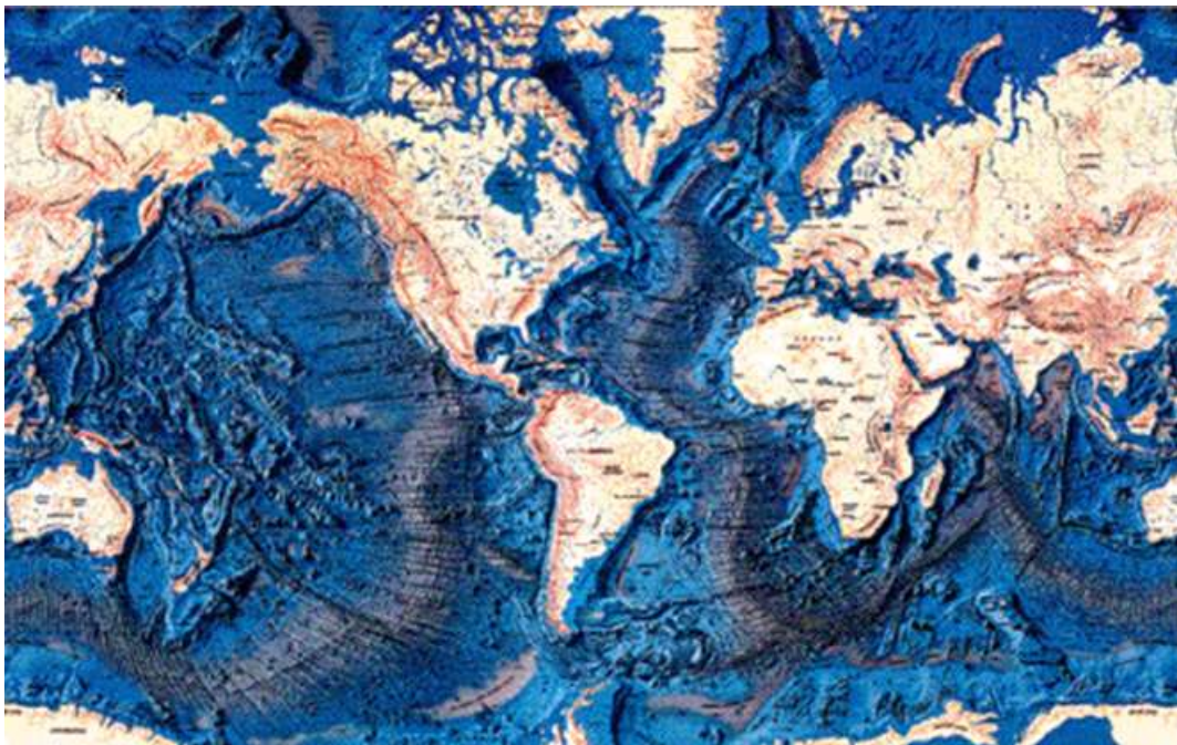
Fig: Mid oceanic Ridges
