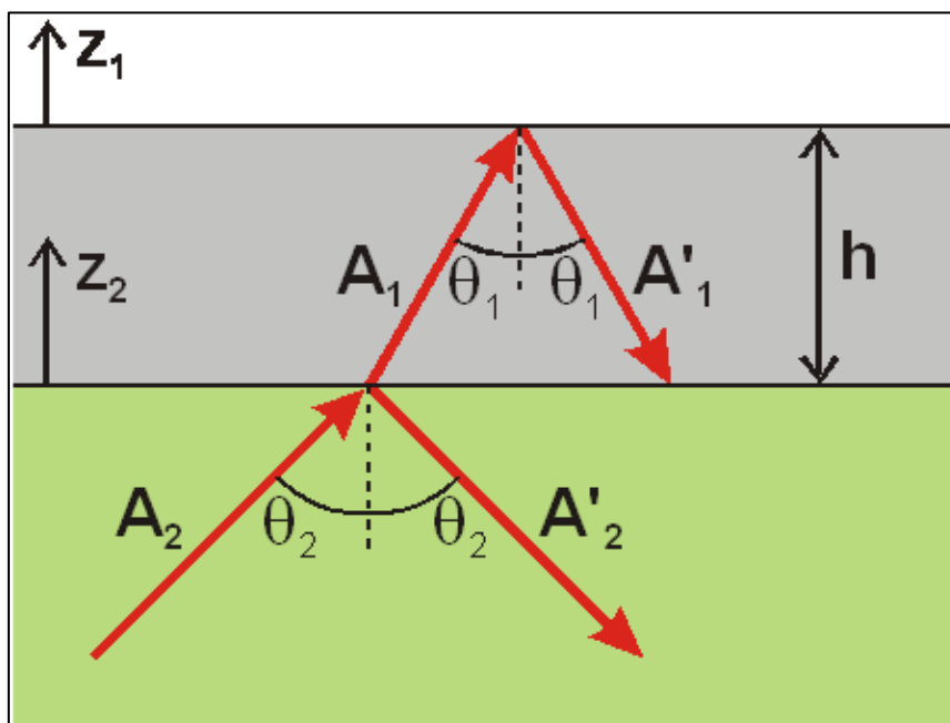
Fig1: Seismic site effects / wave amplification in a horizontal layer (SH-waves): various wavefields.
