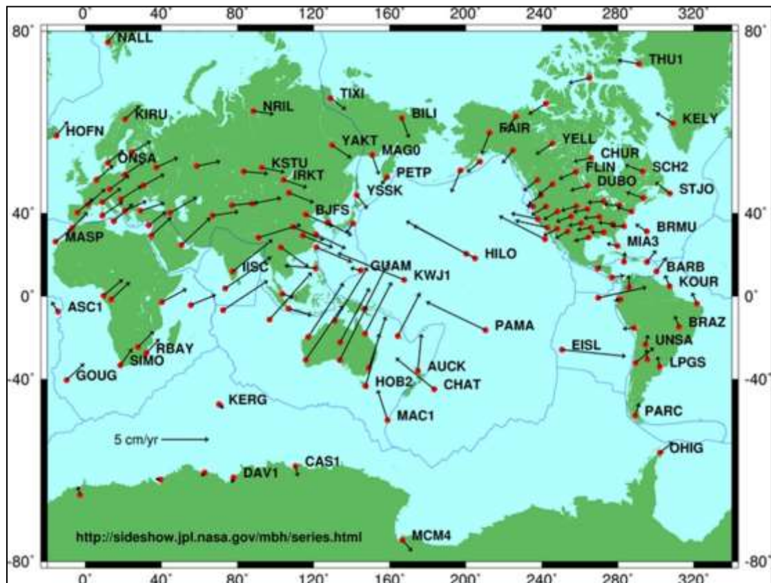
Fig: Movement of global plate boundaries
