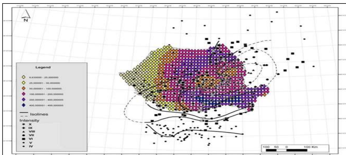
Fig: Seismic hazard determined using the strongest recorded earthquake with magnitude M_w = 7.7 (10th November 1940, Ardeleanu, 2010).
