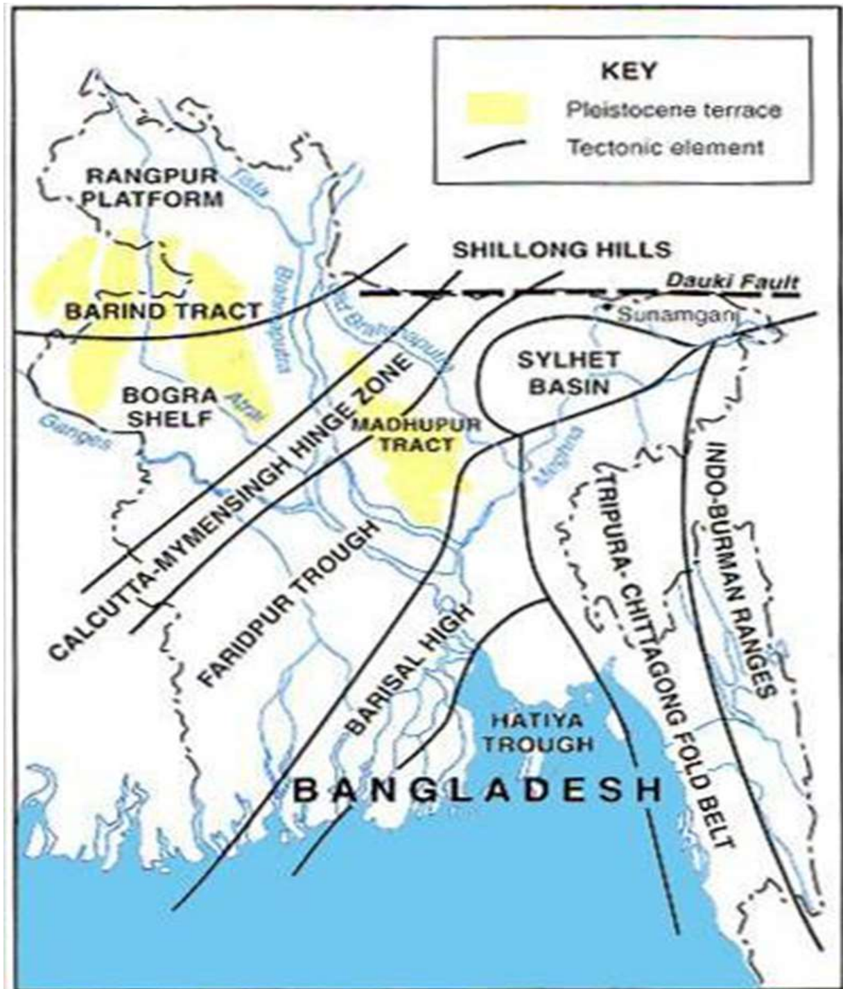
Fig: Tectonic framework of Bangladesh
