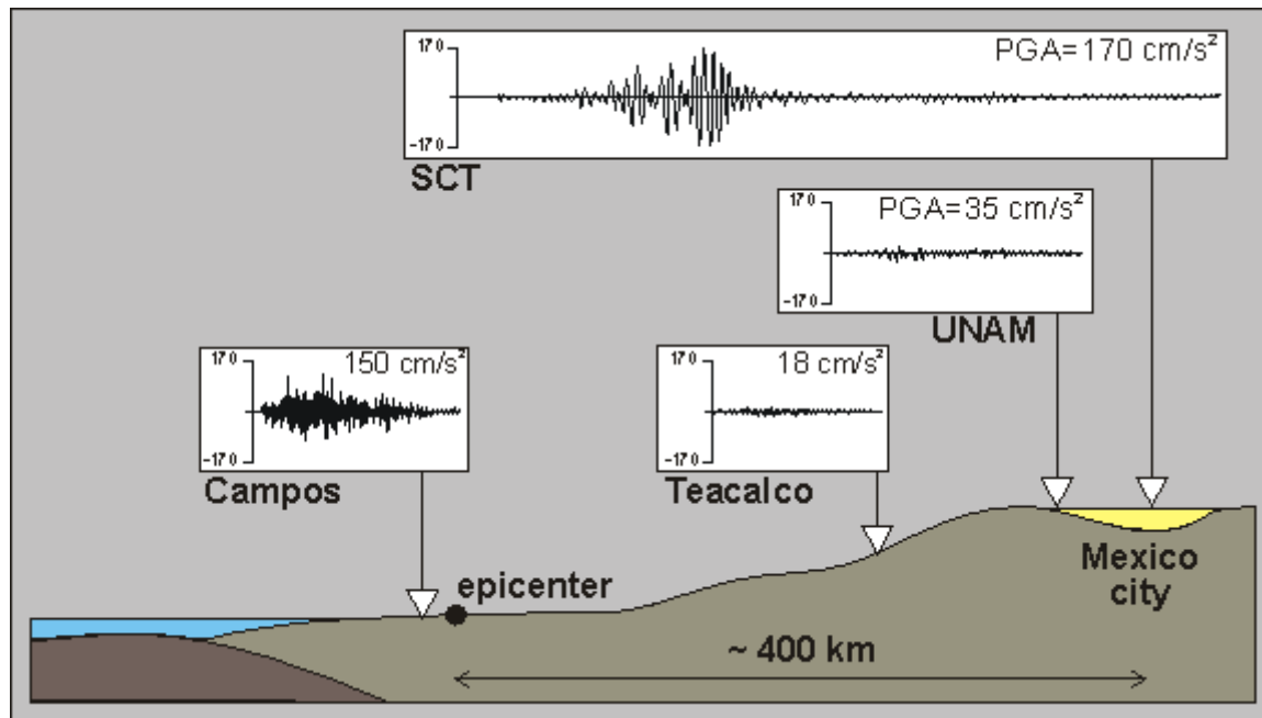
Fig: Site effects in Mexico City: recordings from the 1985 earthquake
