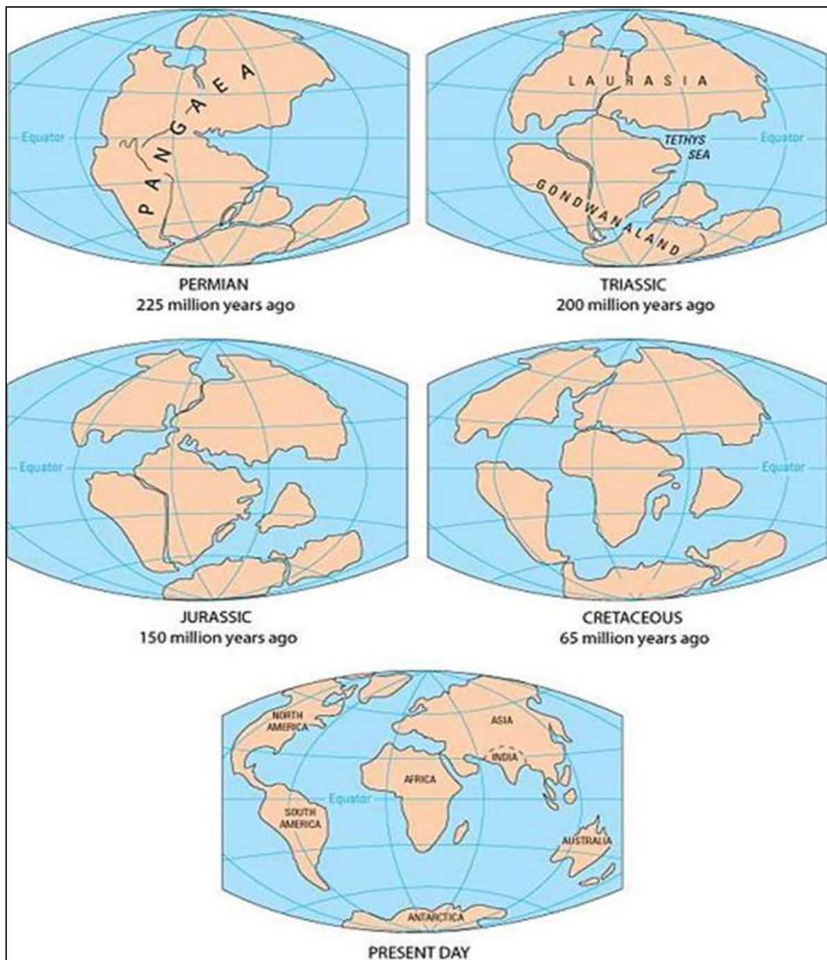
Fig: Maps by Wegener (1915), showing continental drift
