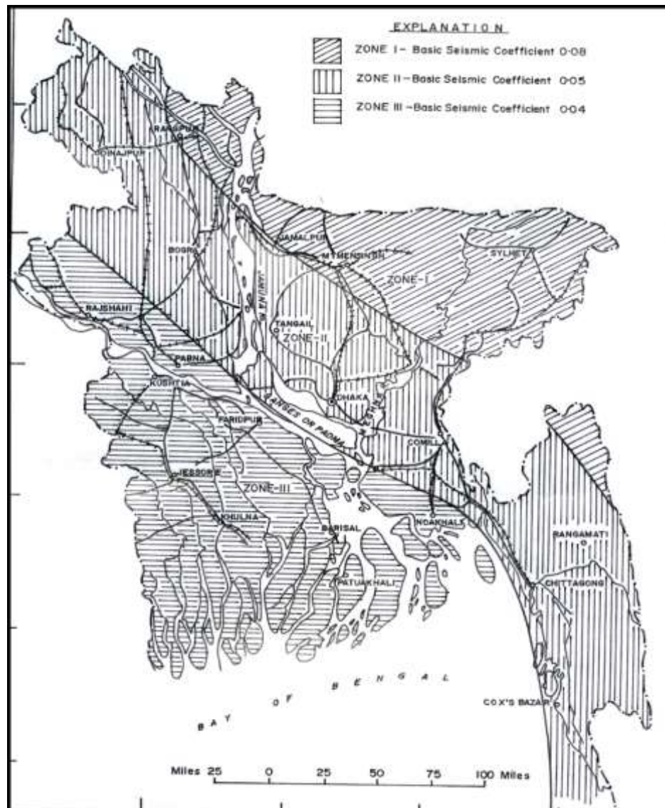
Fig: Seismic Zoning map of Bangladesh (1979)
