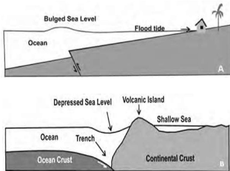
Figure 5 (A) Schematic diagram showing development of local bulge over the sea level because of uplifting of a block of Ocean Crust. This causes flood tide in coastal region. (B)
