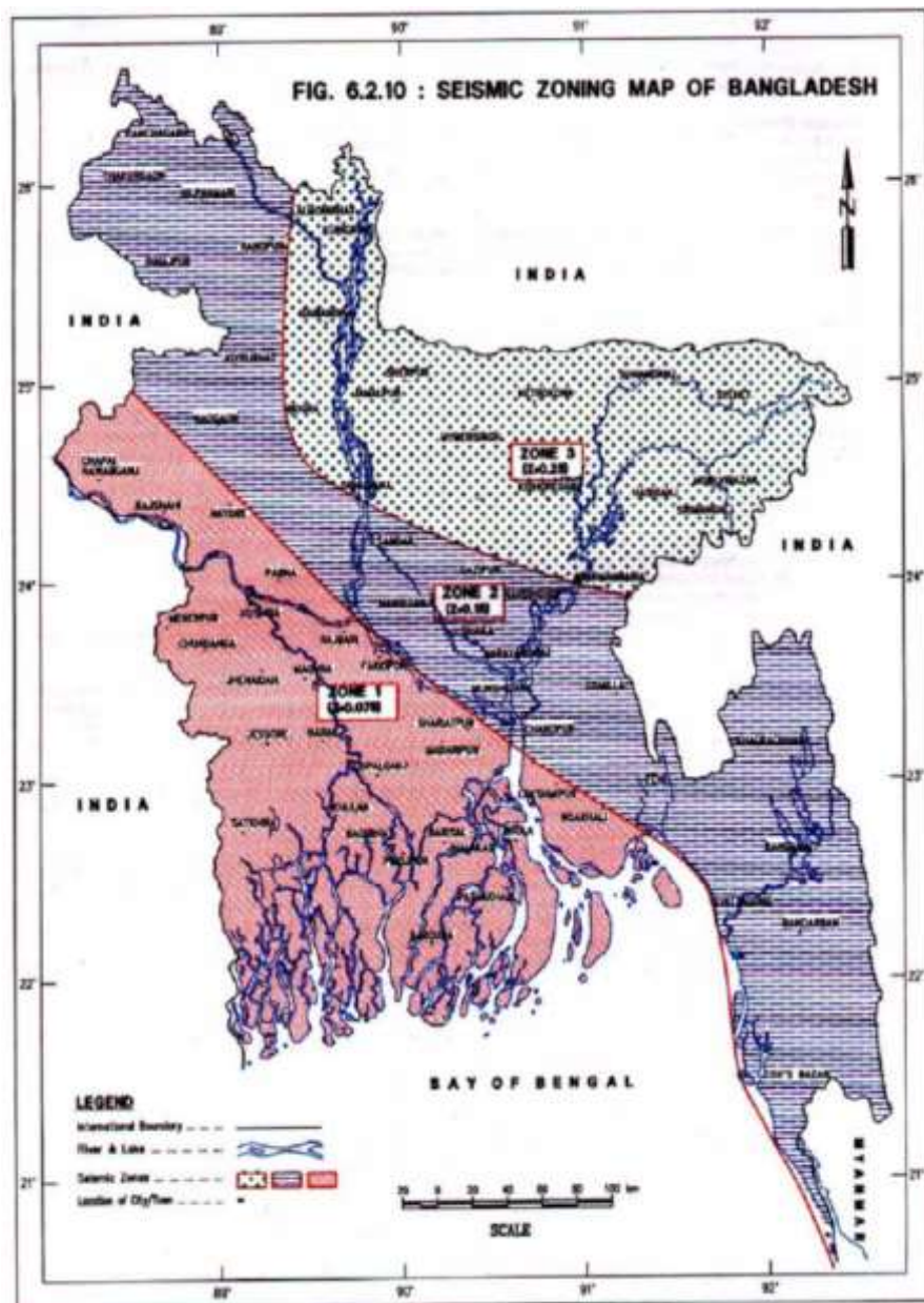
Fig: Seismic Zoning map of Bangladesh (1993)
