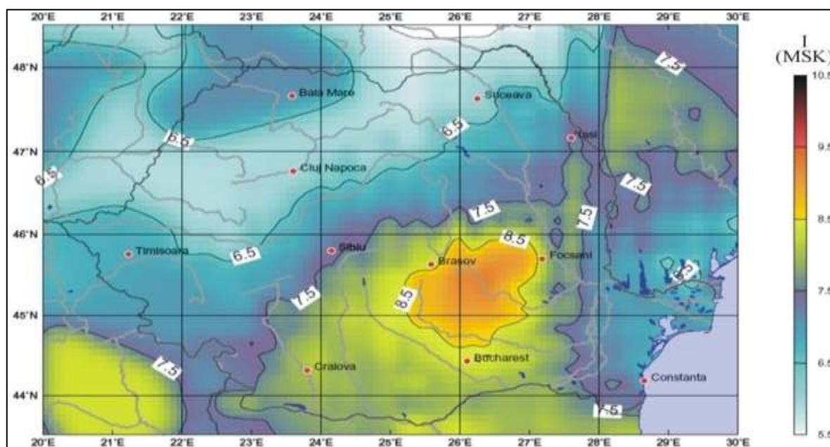
Fig: Probabilistic seismic hazard computed in terms of microseismic intensity (MSK scale), resulted by considering all seismic zones, with a return period of 475 years (Ardeleanu, 2010).
