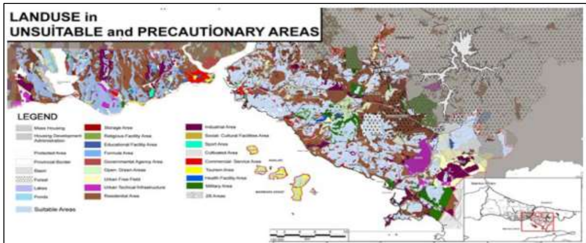
Fig: Landuse in unsuitable and precautionary areas
