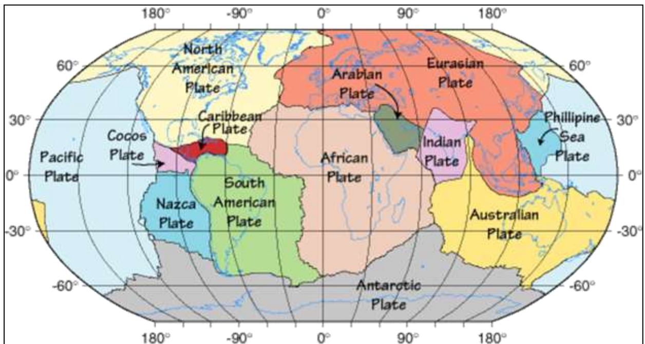
Fig: Tectonic plates of Earth
