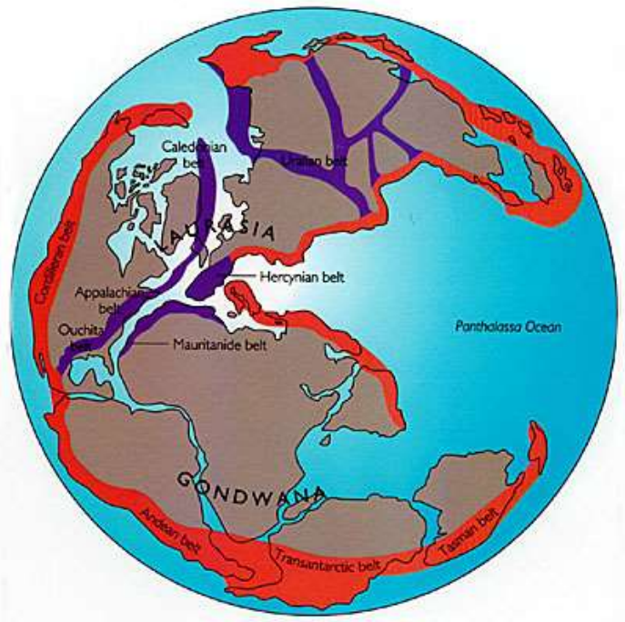
Matching rock types and rock ages
