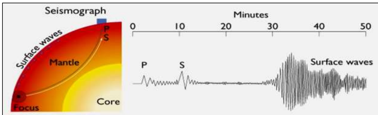
Fig: Illustrations of seismic waves
