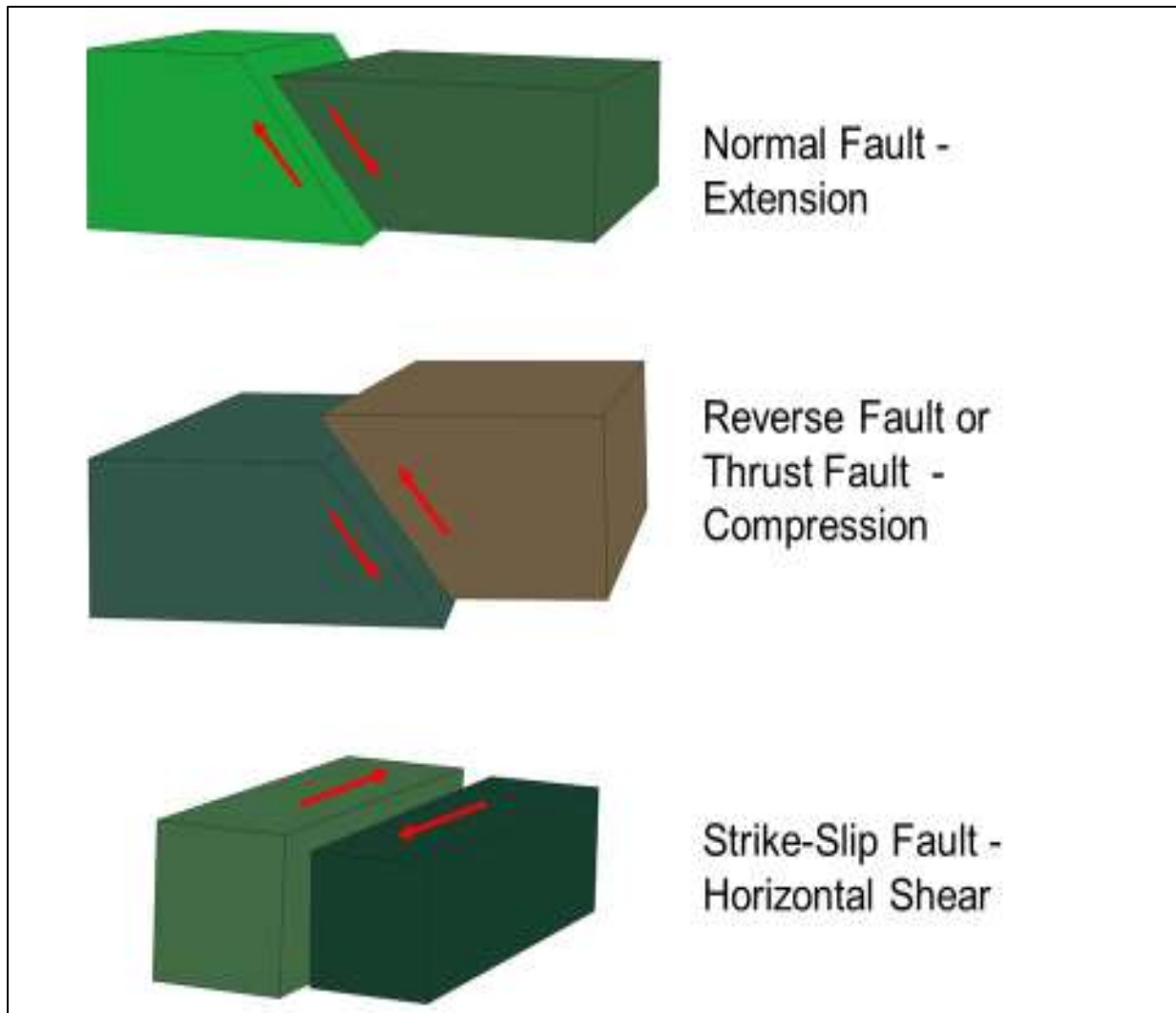
Fig: Different types of Fault
