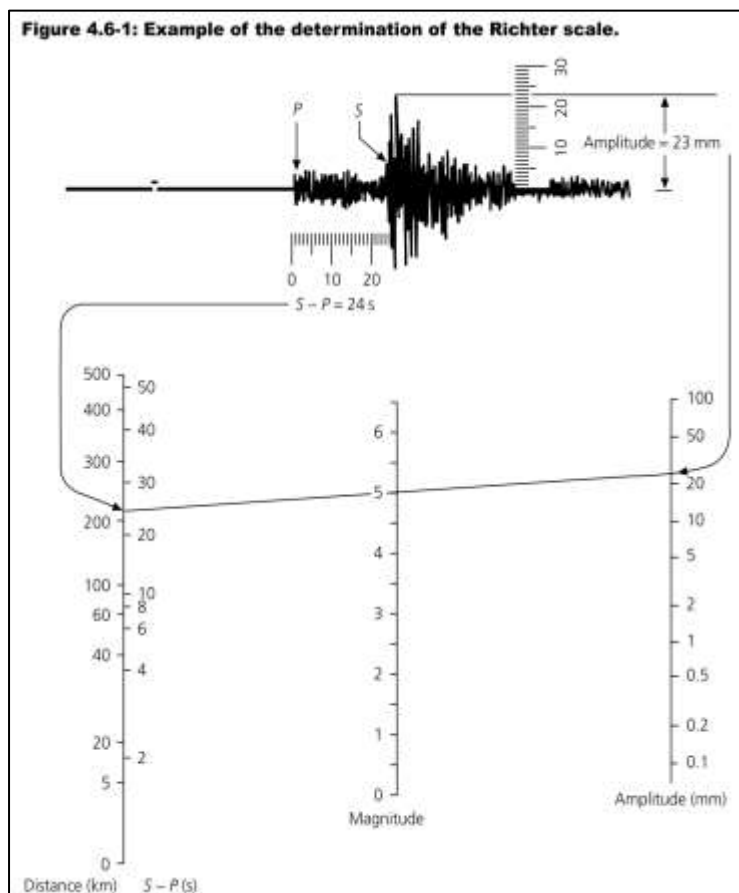
Fig: Graphical procedure of determining Richter magnitude
