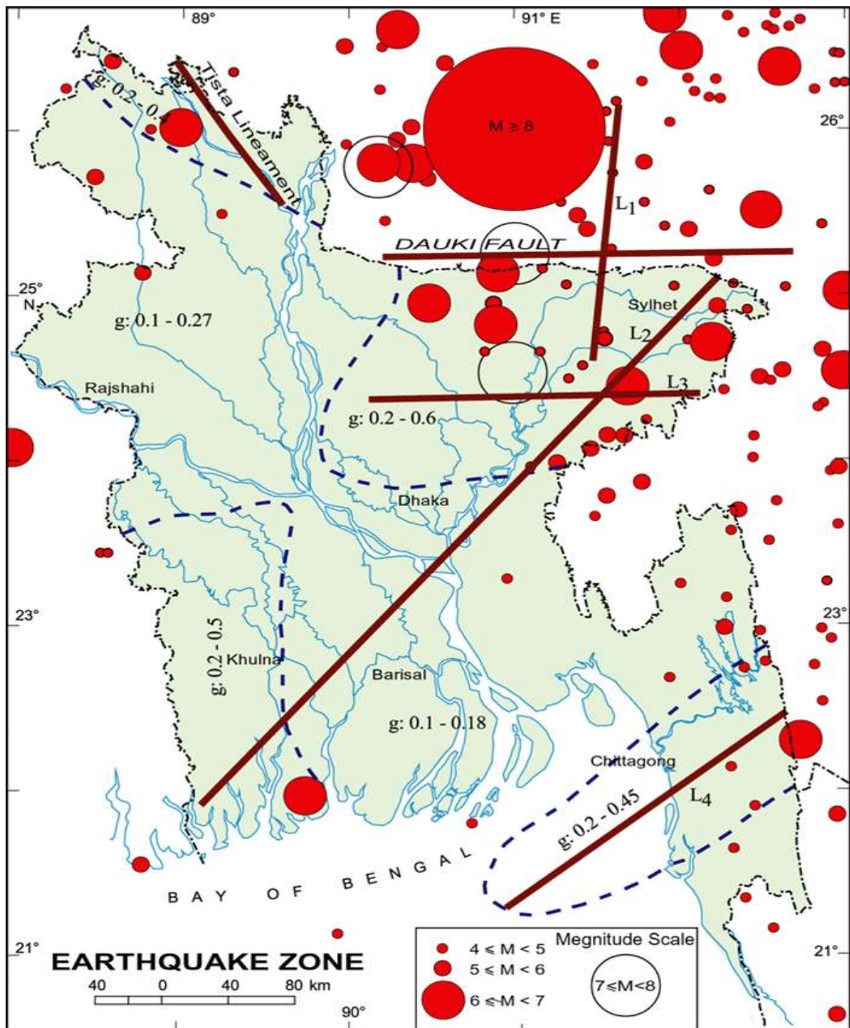
Figure: Location of earthquake epicenters and tectonic elements in and closes vicinity of Bangladesh
