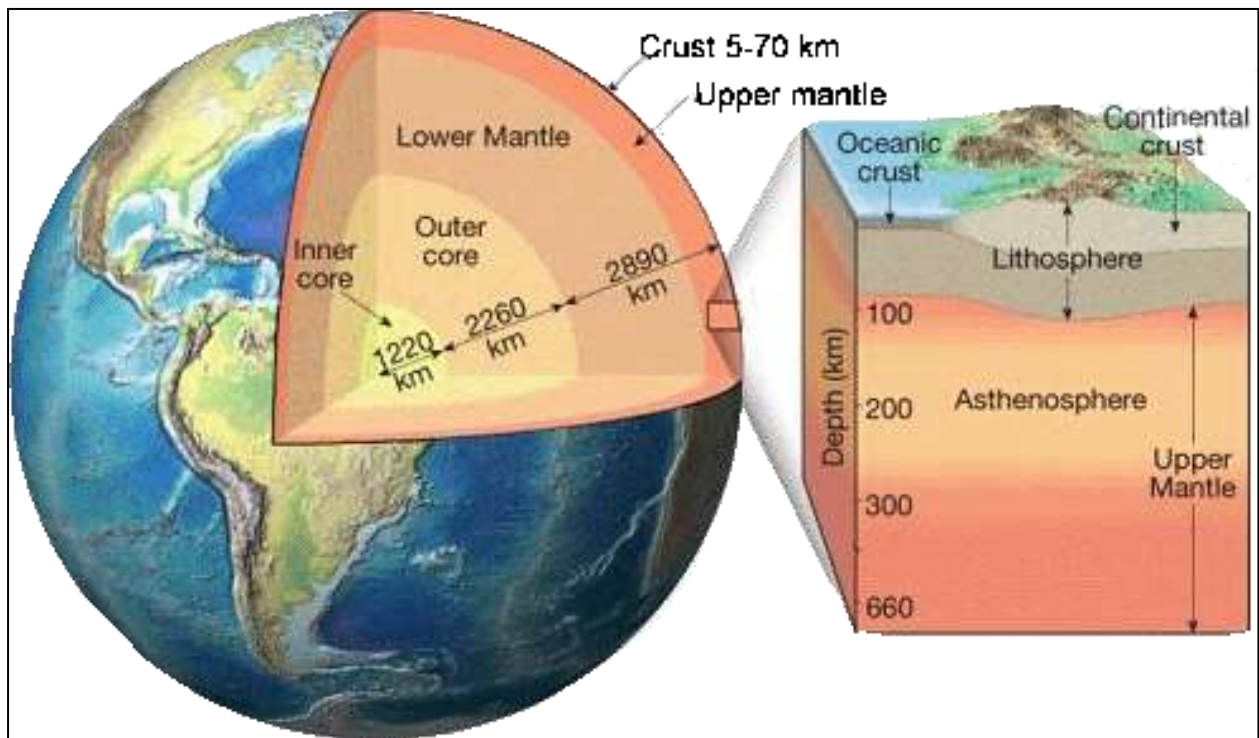
Fig: Earth's Internal Layering
